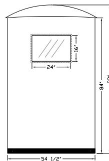
RAIN TENT (Rear)
