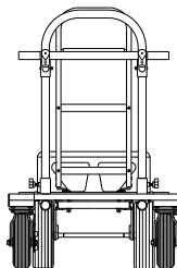
Mag Junior with 30" HD Nose
