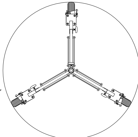
53 7/8" Diameter Circle
