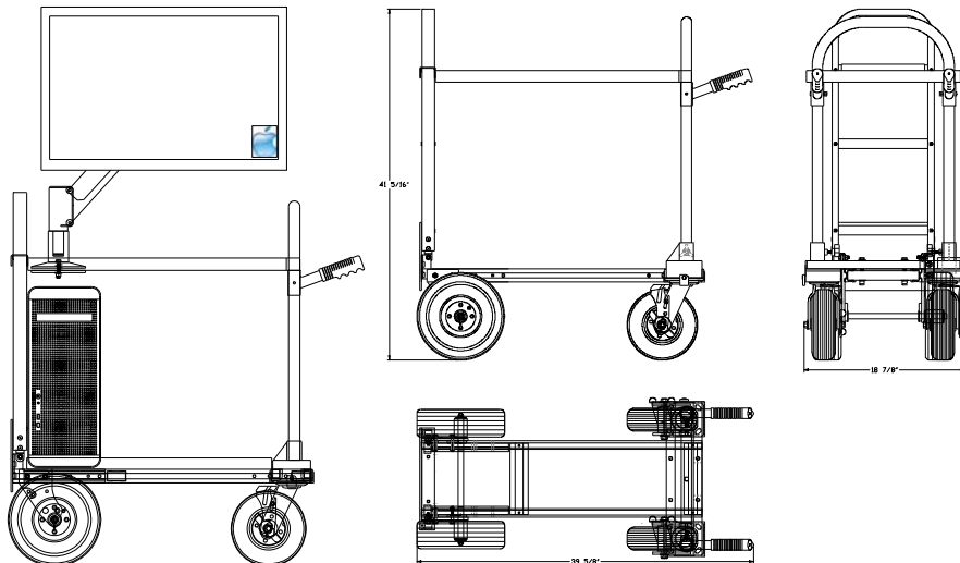
Magliner Mini with Mag LCD Monitor Arm, Mac Pro and 30" Apple Cinema Display (Page 120)
